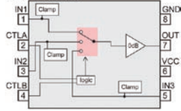
BH76332FVM
