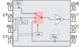
BH76333FVM
