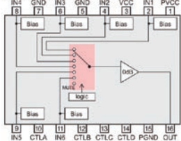
BH76363FV
