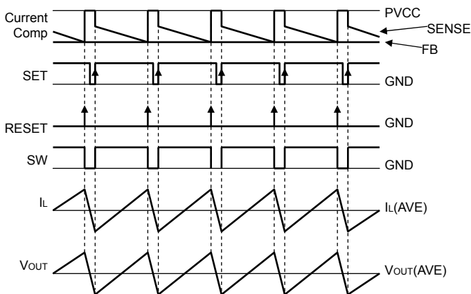
Fig.23 PWM switching timing chart
